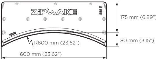
IT600-E TUNNEL R600
