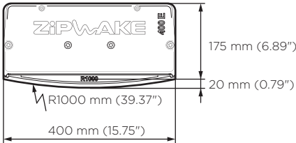
IT400-E ROUND R1000
