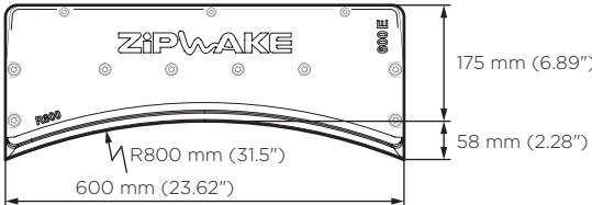
IT600-E TUNNEL R800
