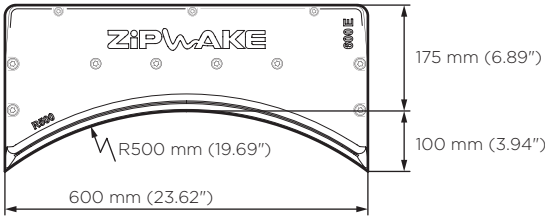
IT600-E TUNNEL R500
